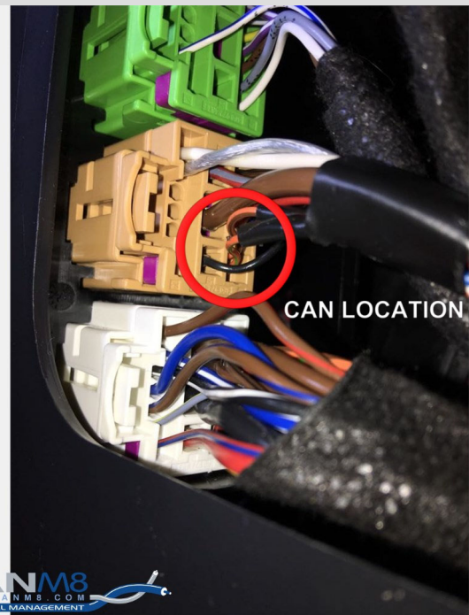
CAN wiring
