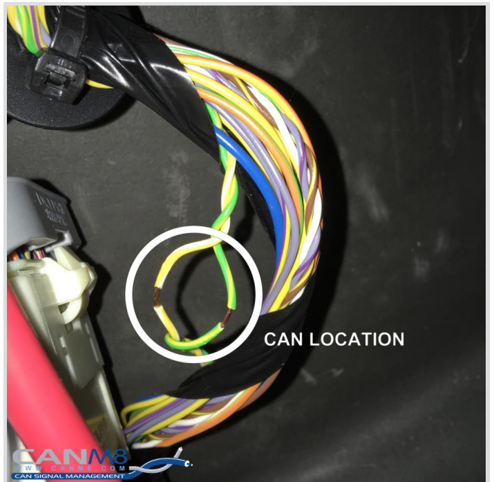
CAN wiring
